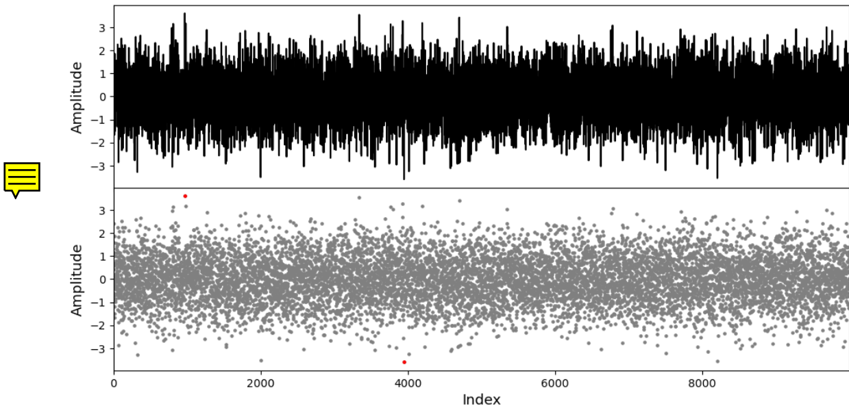
Figure 1: Detection of the two samples (red dots) that do not agree the Probit approach within the 10 000 values composing the synthetic dataset.
